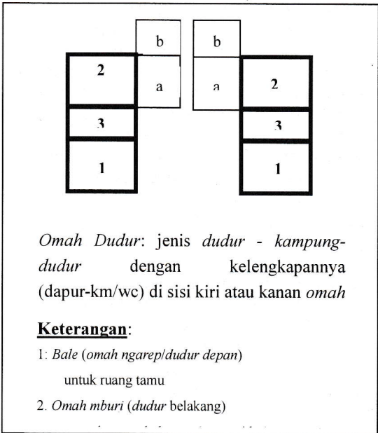
Figure 11. Omah dudur layout pattern: dudur-kampung-dudur Source: Documentation, 2015
