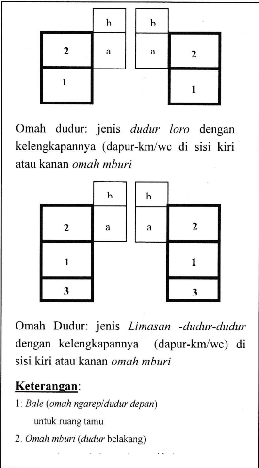
Figure 10. Omah dudur loro layout pattern and limasan-dudur-dudur Source: Documentation, 2015
