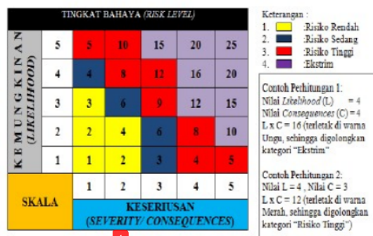
Gambar 1. Risk Matrix
